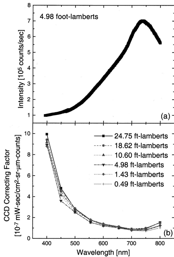
FIG. 3. (a) The CCD spectral response curve for a 4.98 foot-lamberts (17.06 cd/m 2 ) luminance reading. (b) The CCD correction curves for different attenuator settings.
